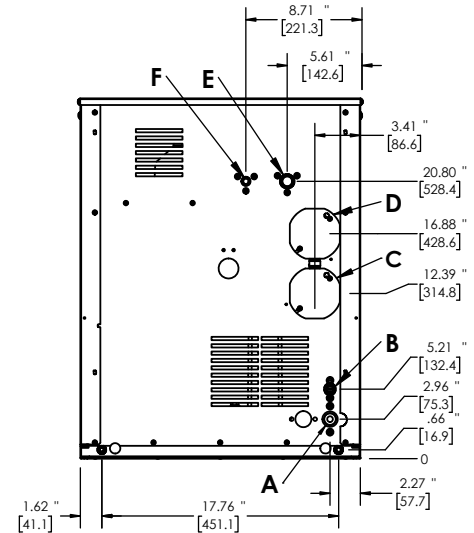
UTILITIES / BACK VIEW
