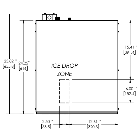
PLAN / TOP VIEW
