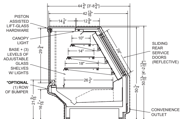
Section View
