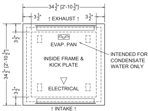
Plan Mechanical View
