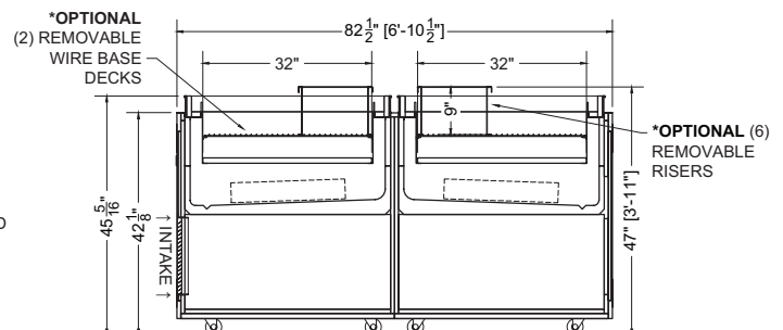
Section B:B View
