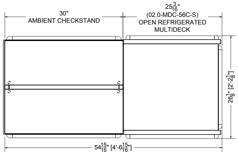
Plan Mechanical View
