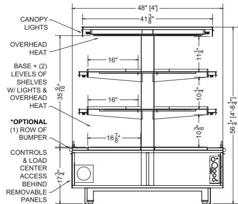
Section View
